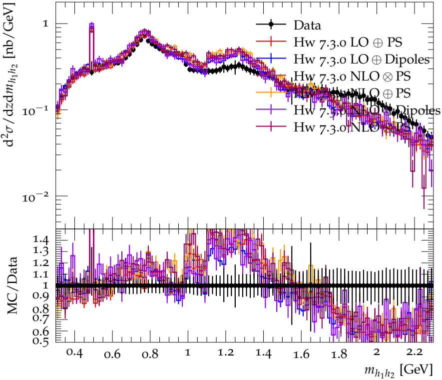
Differential cross section for \pi^+\pi^- ( 0.75 < z < 0.8 ) (strong)
