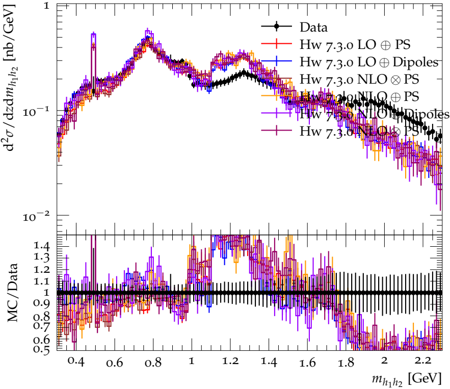
Differential cross section for \pi^+\pi^- ( 0.8 < z < 0.85 ) (strong)
