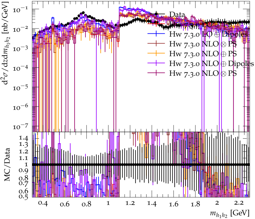
Differential cross section for \pi^+\pi^- ( 0.95 < z < 1. ) (strong)
