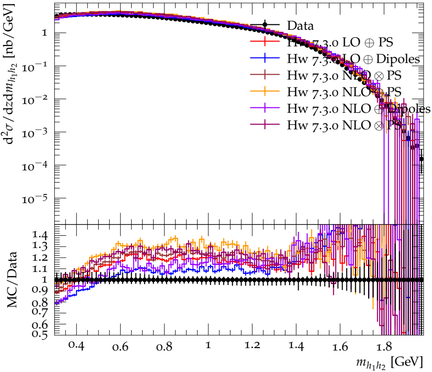
Differential cross section for \pi^+\pi^+ ( 0.35 < z < 0.4 ) (strong)
