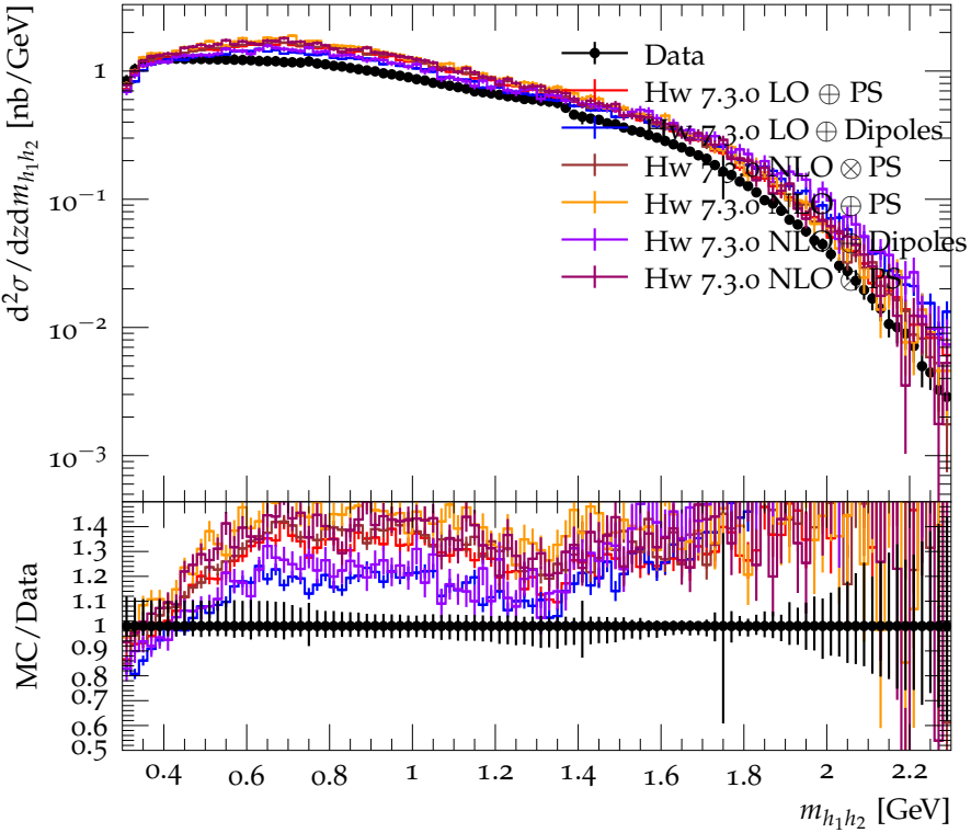
Differential cross section for \pi^+\pi^+ ( 0.5 < z < 0.55 ) (strong)
