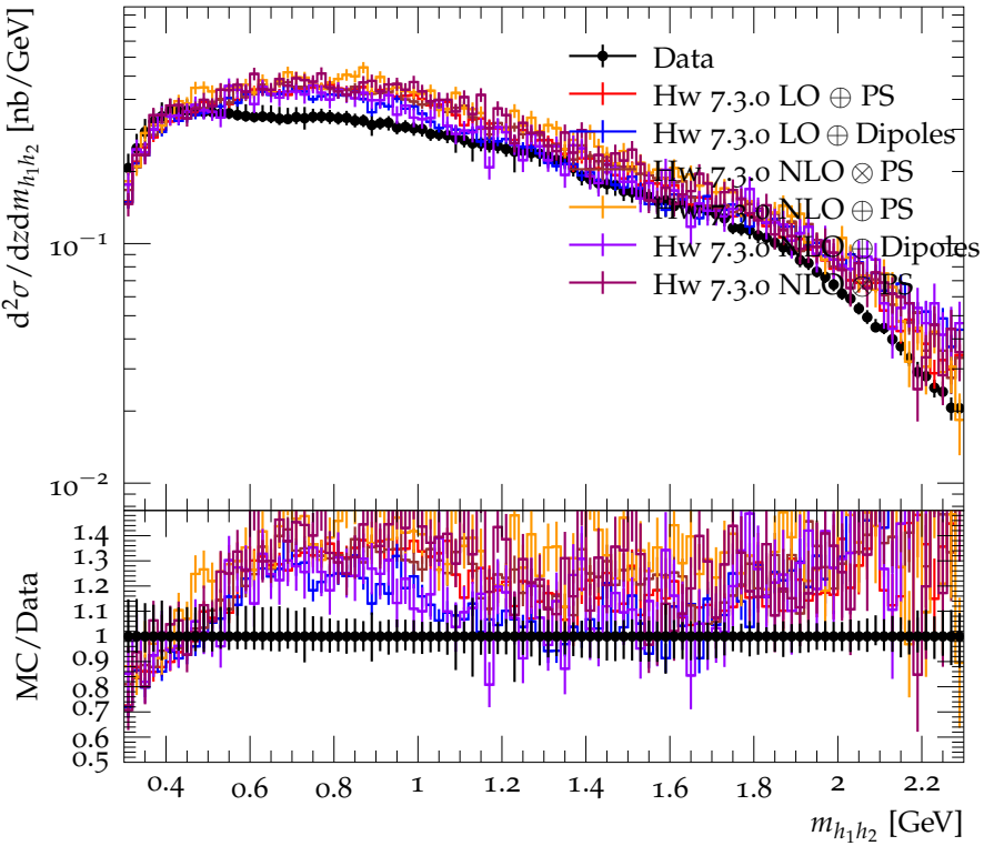
Differential cross section for \pi^+\pi^+ ( 0.65 < z < 0.7 ) (strong)
