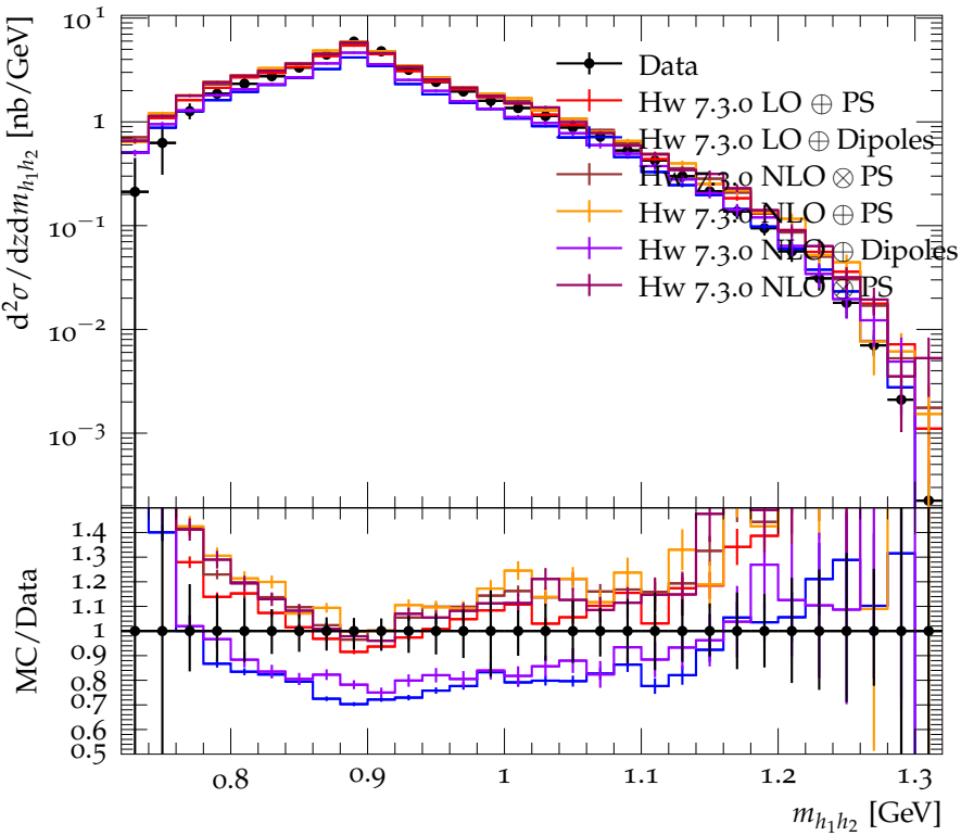
Differential cross section for \pi^+K^- ( 0.2 < z < 0.25 ) (strong)
