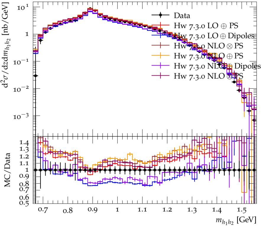
Differential cross section for \pi^+K^- ( 0.25 < z < 0.3 ) (strong)
