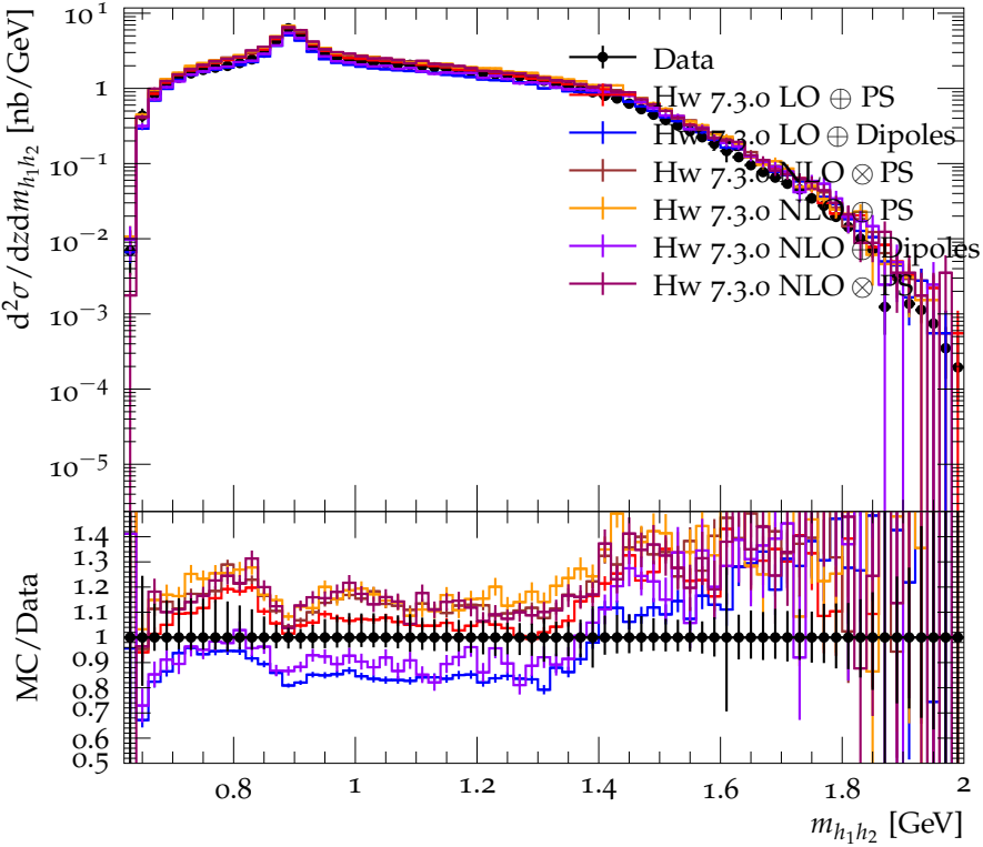
Differential cross section for \pi^+K^- ( 0.35 < z < 0.4 ) (strong)
