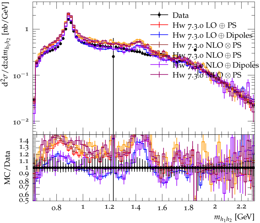
Differential cross section for \pi^+K^- ( 0.6 < z < 0.65 ) (strong)
