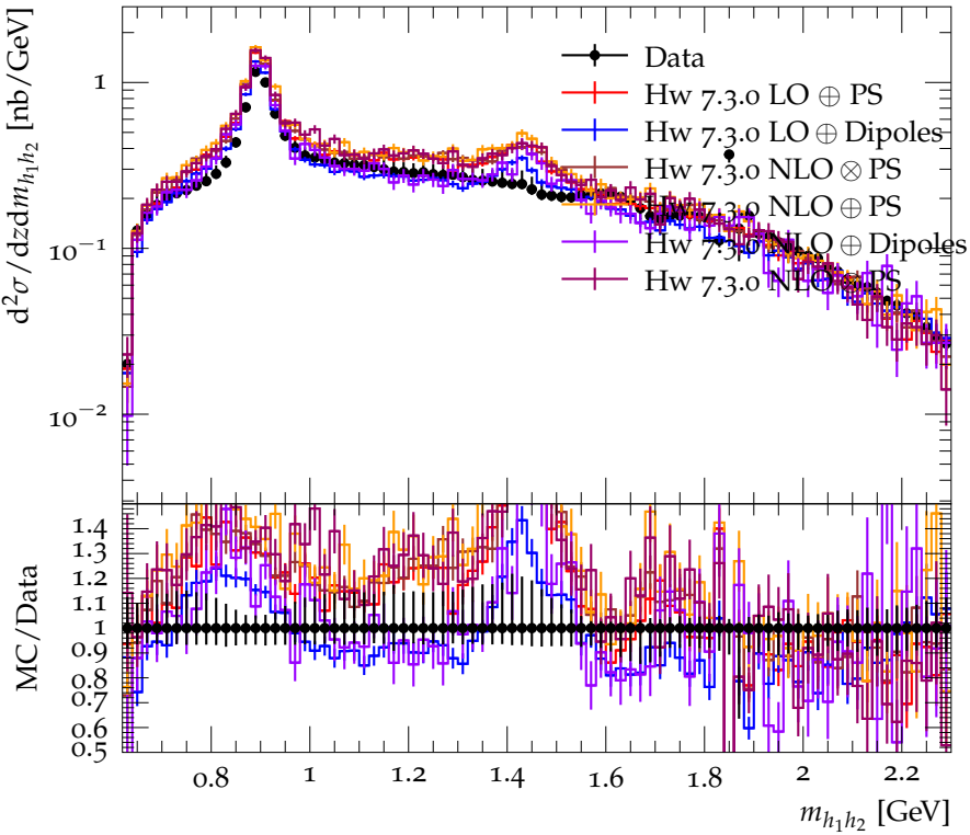
Differential cross section for \pi^+K^- ( 0.65 < z < 0.7 ) (strong)
