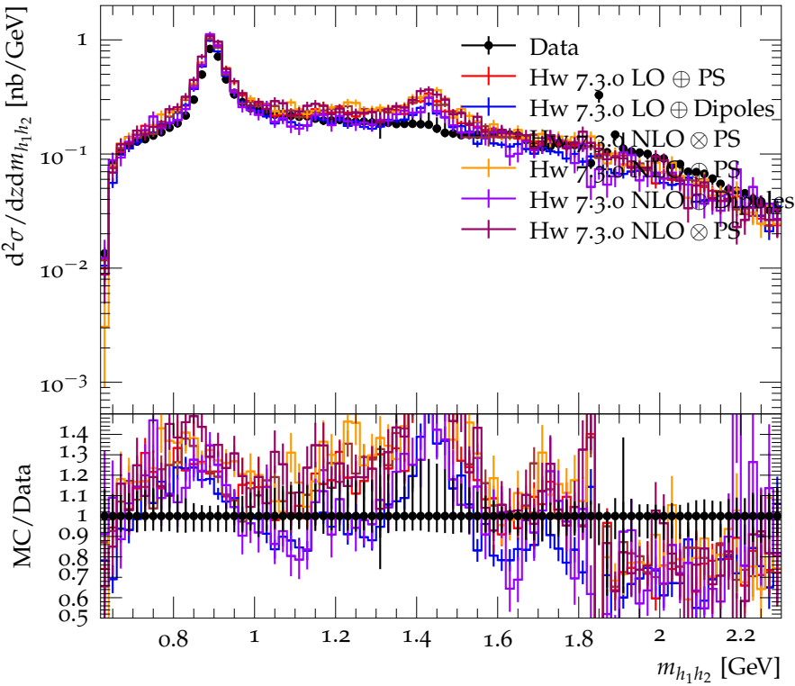
Differential cross section for \pi^+K^- ( 0.7 < z < 0.75 ) (strong)
