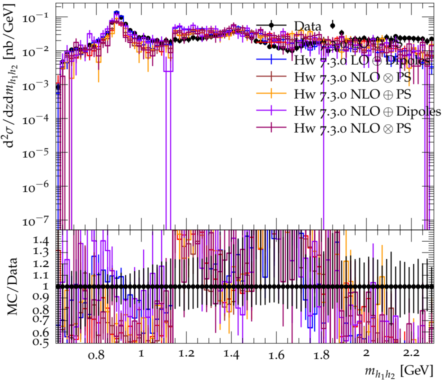
Differential cross section for \pi^+K^- ( 0.9 < z < 0.95 ) (strong)
