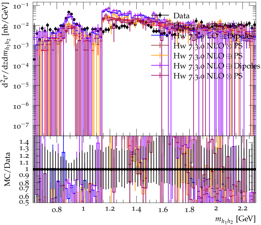
Differential cross section for \pi^+K^- ( 0.95 < z < 1. ) (strong)
