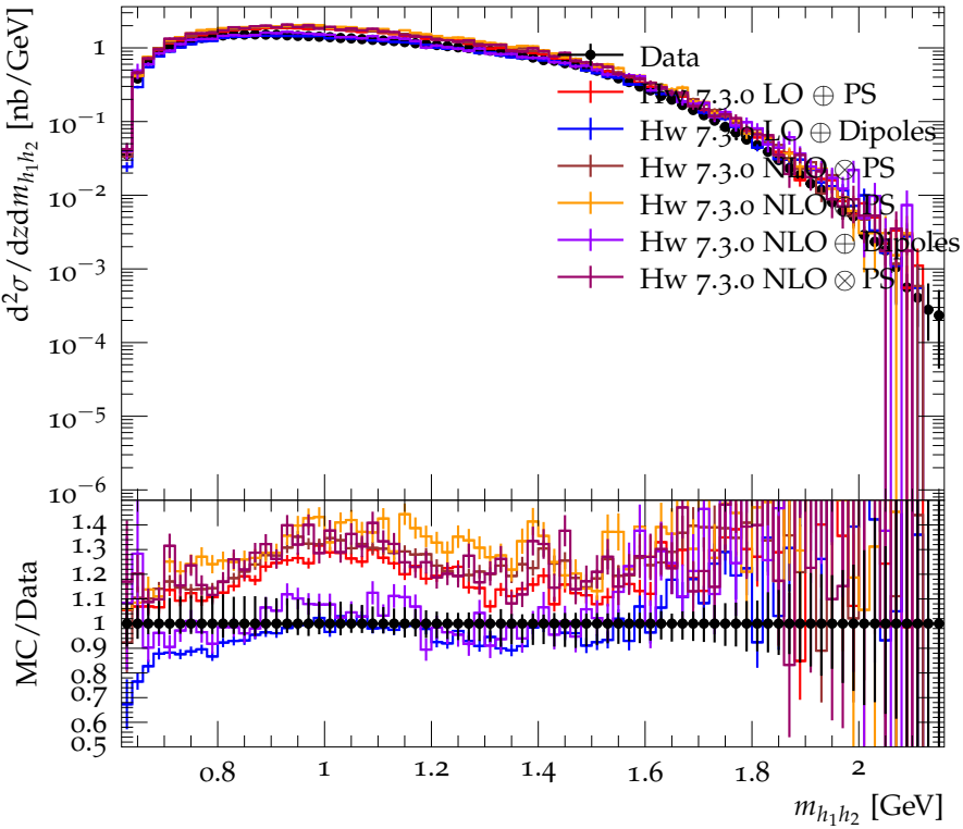
Differential cross section for \pi^+K^+ ( 0.4 < z < 0.45 ) (strong)
