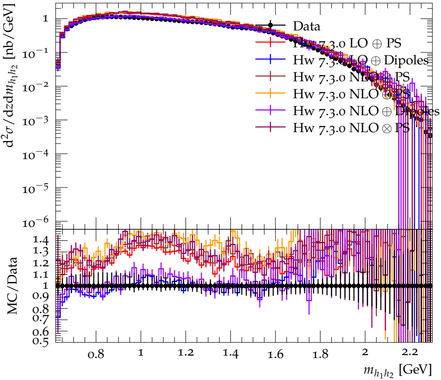
Differential cross section for \pi^+K^+ ( 0.45 < z < 0.5 ) (strong)
