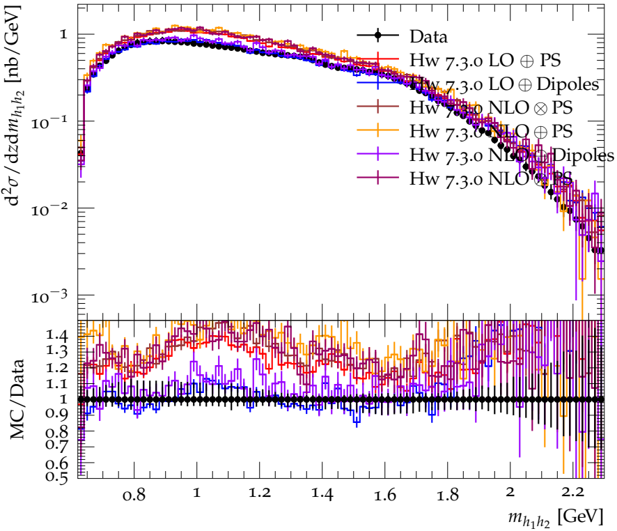
Differential cross section for \pi^+K^+ ( 0.5 < z < 0.55 ) (strong)
