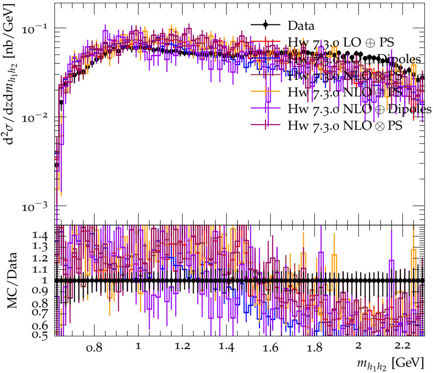
Differential cross section for \pi^+K^+ ( 0.8 < z < 0.85 ) (strong)
