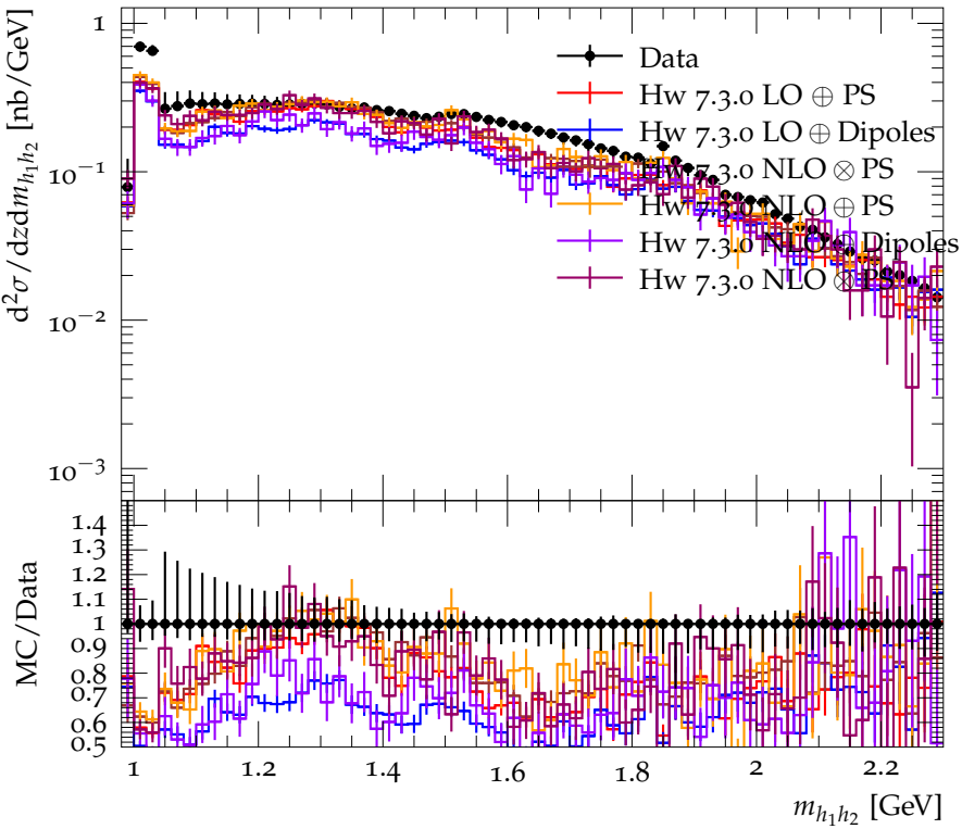
Differential cross section for K^+K^- ( 0.6 < z < 0.65 ) (strong)
