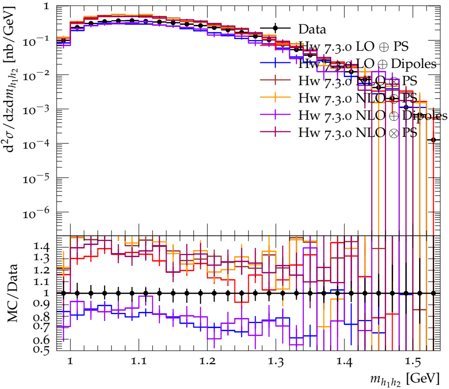
Differential cross section for K^+K^+ ( 0.25 < z < 0.3 ) (strong)
