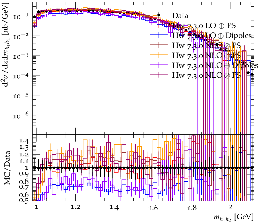
Differential cross section for K^+K^+ ( 0.4 < z < 0.45 ) (strong)
