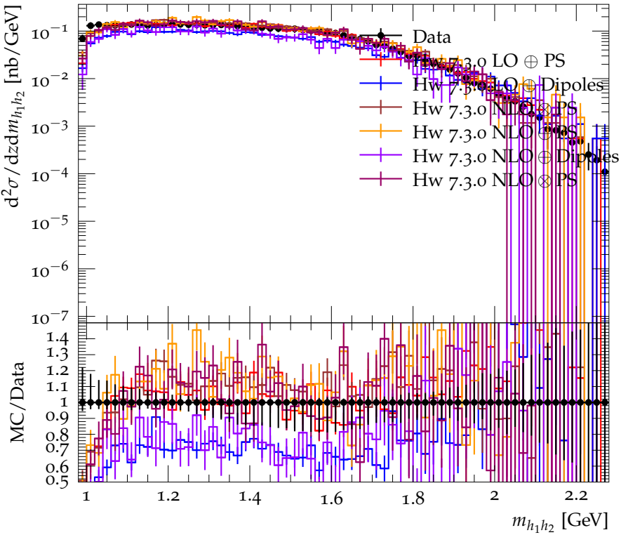
Differential cross section for K^+K^+ ( 0.45 < z < 0.5 ) (strong)
