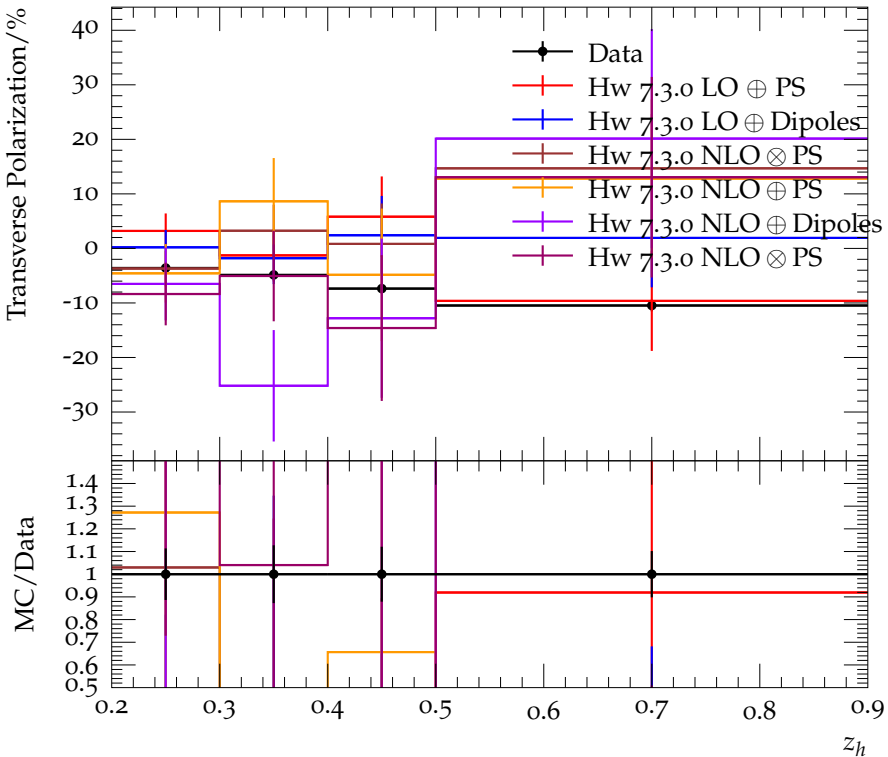
Transverse \bar{\Lambda}^0 polarization for 0.2 < z_\Lambda < 0.3 and opposite \pi^-
