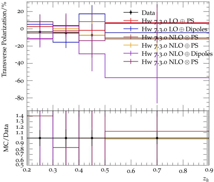
Transverse \bar{\Lambda}^0 polarization for 0.2 < z_\Lambda < 0.3 and opposite K^-
