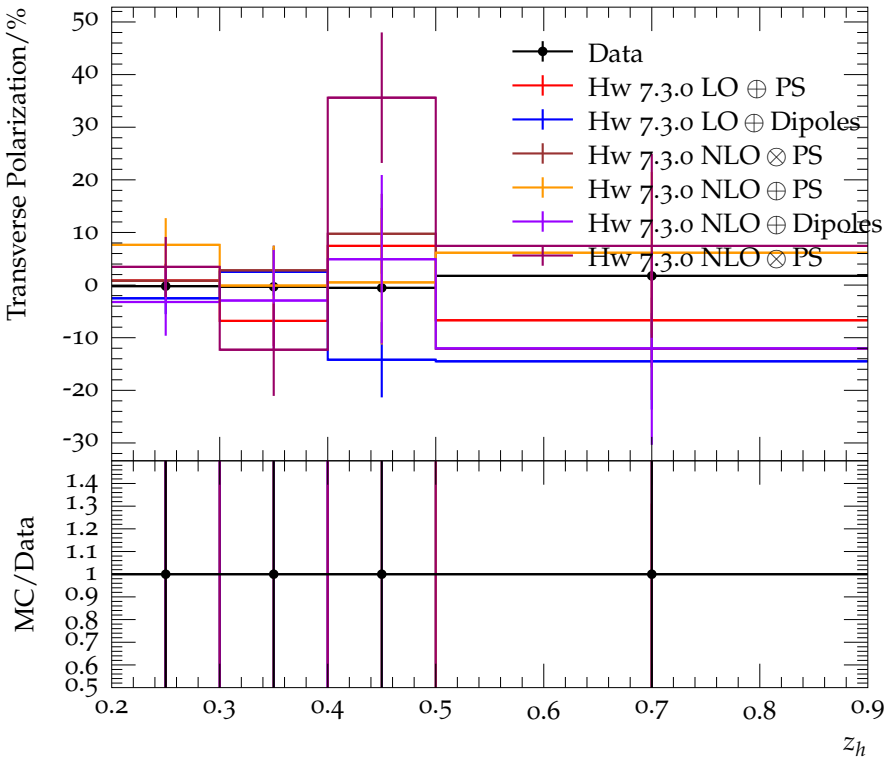
Transverse \Lambda^0 polarization for 0.3 < z_\Lambda < 0.4 and opposite \pi^-
