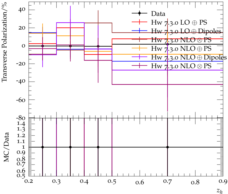
Transverse \Lambda^0 polarization for 0.3 < z_\Lambda < 0.4 and opposite K^-
