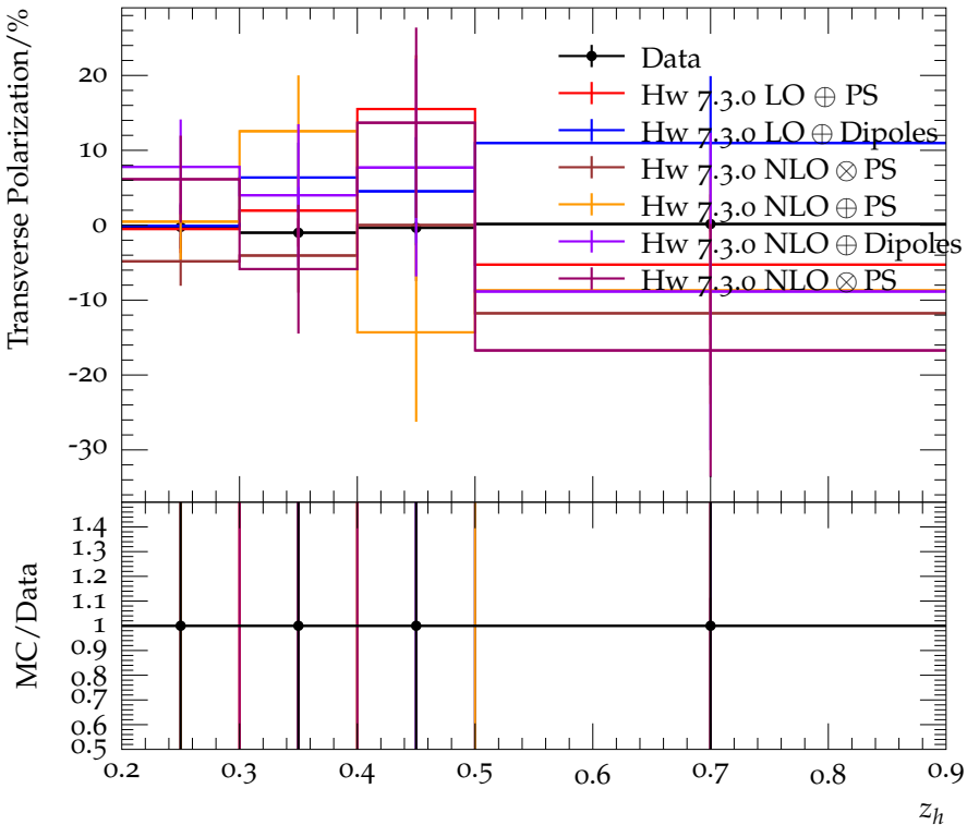
Transverse \bar{\Lambda}^0 polarization for 0.3 < z_\Lambda < 0.4 and opposite \pi^+
