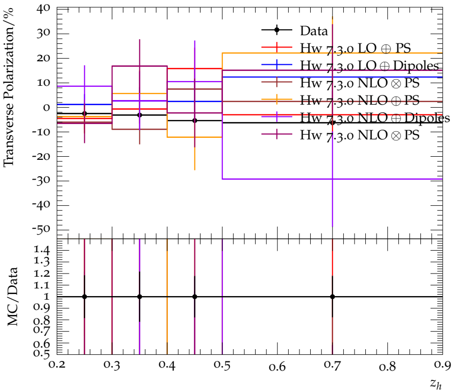
Transverse \bar{\Lambda}^0 polarization for 0.3 < z_\Lambda < 0.4 and opposite K^-
