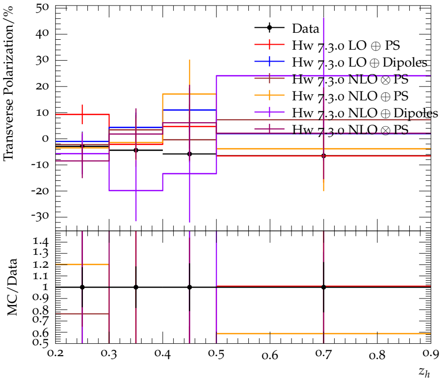
Transverse \Lambda^0 polarization for 0.4 < z_\Lambda < 0.5 and opposite \pi^+
