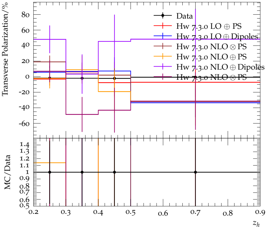
Transverse \bar{\Lambda}^0 polarization for 0.4 < z_\Lambda < 0.5 and opposite K^+
