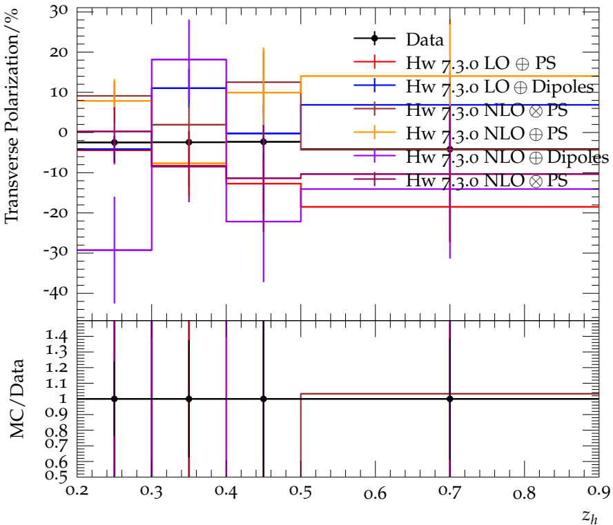
Transverse \Lambda^0 polarization for 0.5 < z_\Lambda < 0.9 and opposite \pi^-
