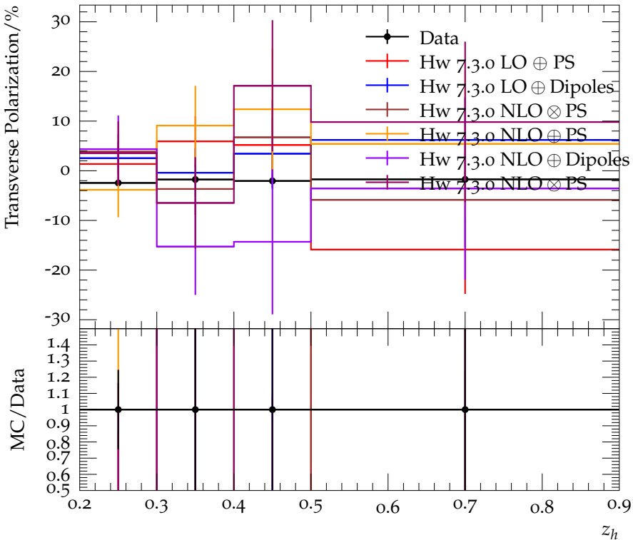
Transverse \bar{\Lambda}^0 polarization for 0.5 < z_\Lambda < 0.9 and opposite \pi^+
