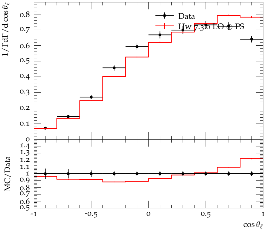
\cos \theta_\ell distribution for B^0 \rightarrow D^{*-} e^+ \nu_e
