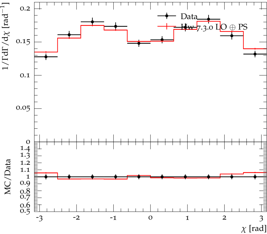
\chi distribution for B^0 \rightarrow D^{*-}e^+\nu_e
