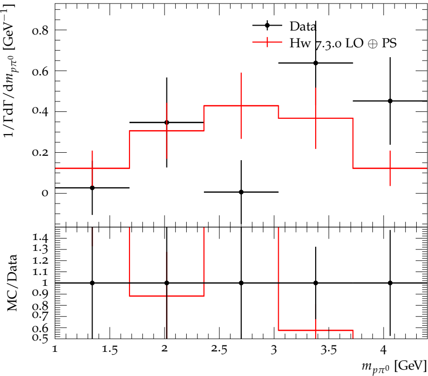
p\pi^0 mass distribution in B^0 \rightarrow p\bar{p}\pi^0
