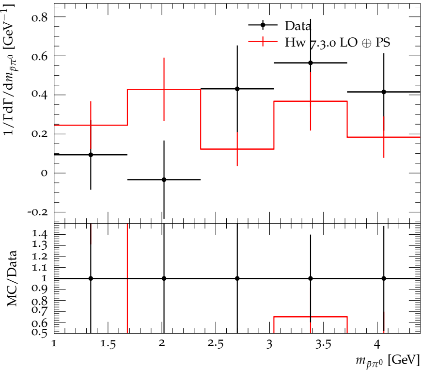
\bar{p}\pi^0 mass distribution in B^0 \rightarrow p\bar{p}\pi^0
