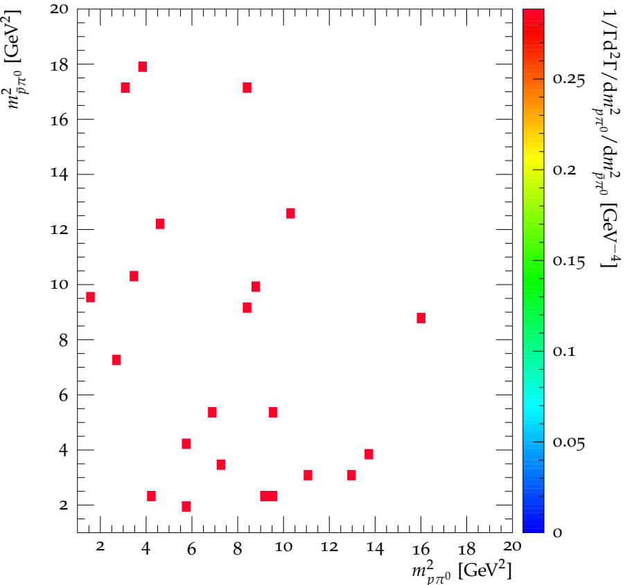
Dalitz plot for B^0 \rightarrow p\bar{p}\pi^0
