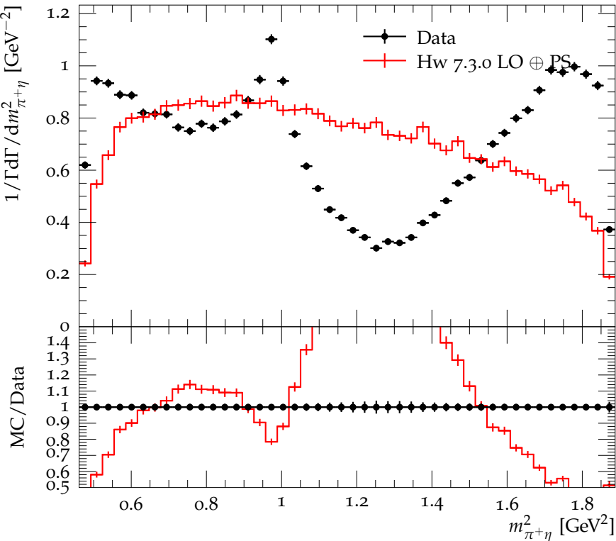
\pi^+\eta mass distribution in D^0 \rightarrow K^-\pi^+\eta
