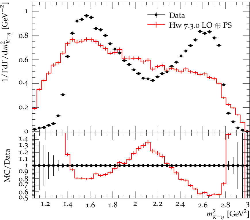
K^- \eta mass distribution in D^0 \rightarrow K^- \pi^+ \eta
