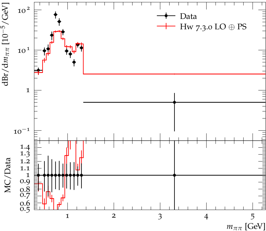
m_{\pi\pi} distribution in B^+ \rightarrow \pi^+ \pi^- \ell^+ \bar{\nu} decays
