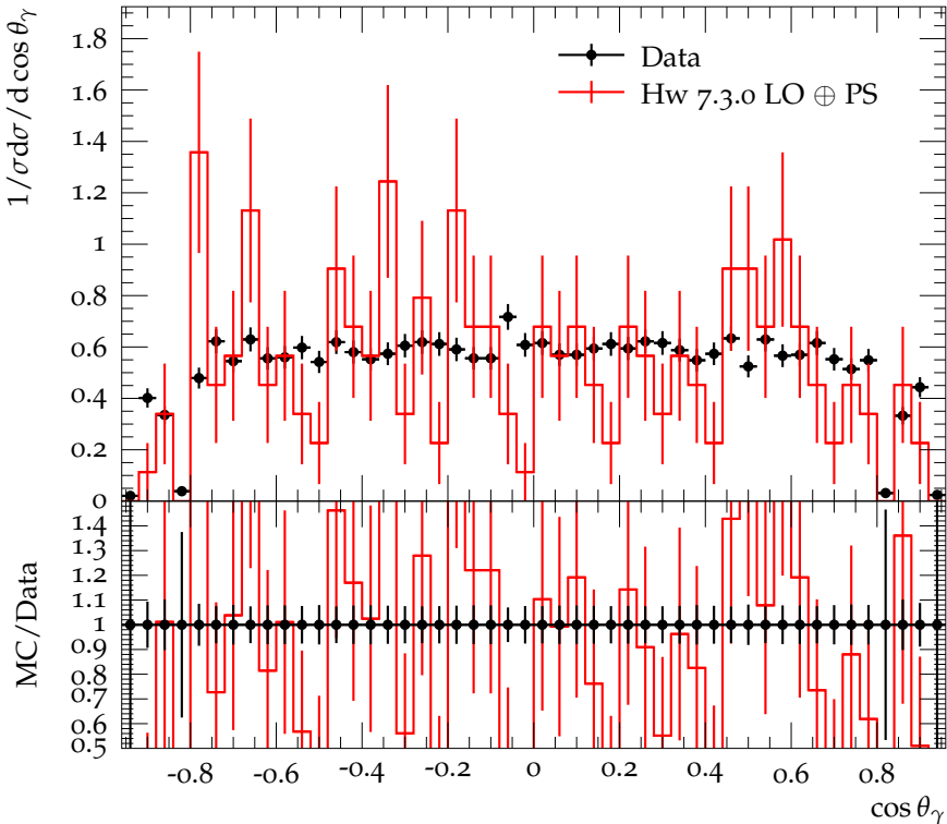
\cos \theta_\gamma distribution for \chi_{c2} production with \chi_{c2} \rightarrow \pi^+ \pi^-
