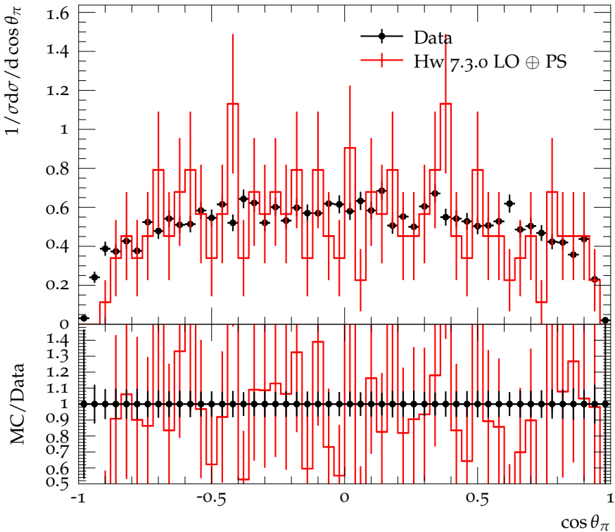
\cos \theta_\pi distribution for \chi_{c2} production with \chi_{c2} \rightarrow \pi^+ \pi^-
