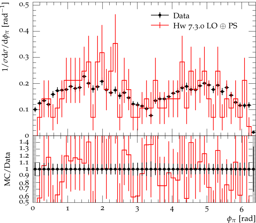
\phi_\pi distribution for \chi_{c2} production with \chi_{c2} \rightarrow \pi^+\pi^-
