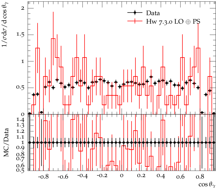
\cos \theta_\gamma distribution for \chi_{c2} production with \chi_{c2} \rightarrow K^+ K^-
