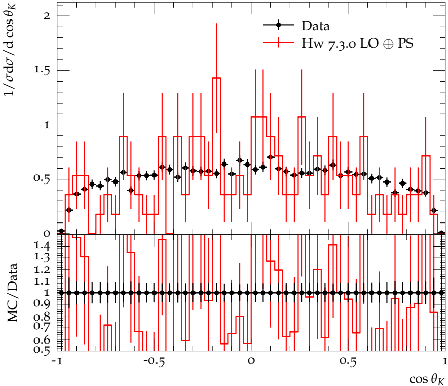
\cos \theta_K distribution for \chi_{c2} production with \chi_{c2} \rightarrow K^+ K^-
