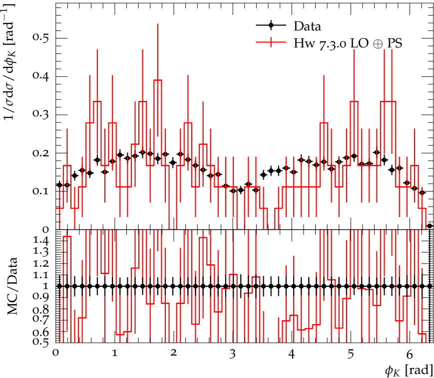
\phi_K distribution for \chi_{c2} production with \chi_{c2} \rightarrow K^+K^-
