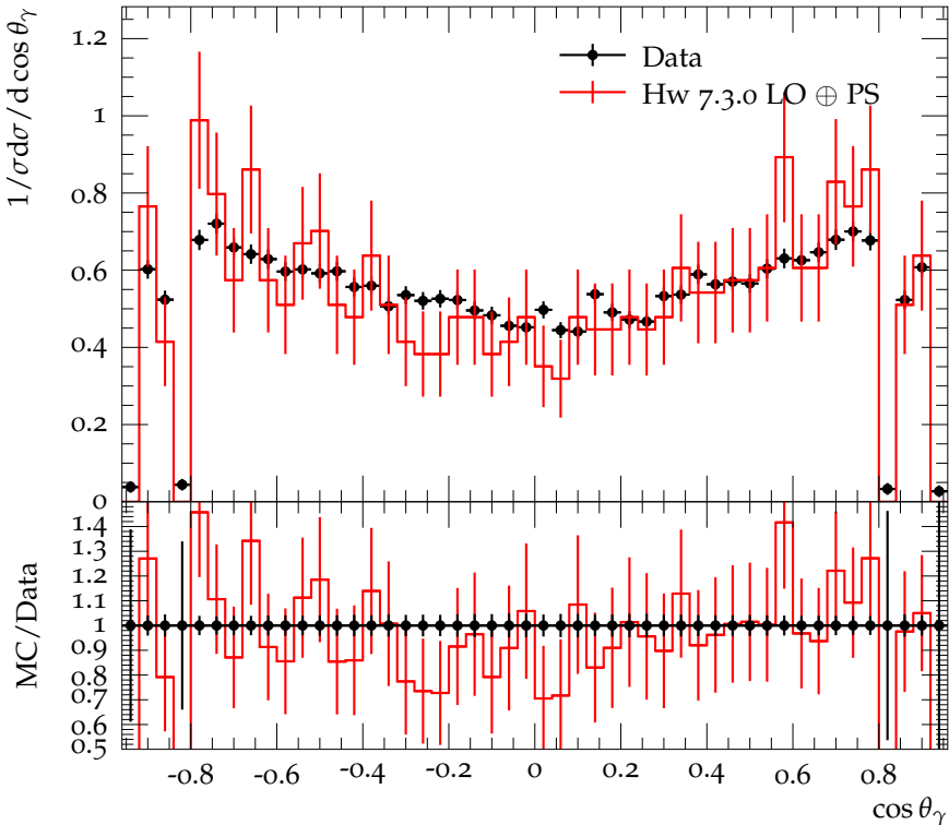
\cos \theta_\gamma distribution for \chi_{c0} production with \chi_{c0} \rightarrow \pi^+ \pi^-
