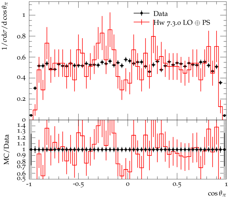
\cos \theta_\pi distribution for \chi_{c0} production with \chi_{c0} \rightarrow \pi^+ \pi^-
