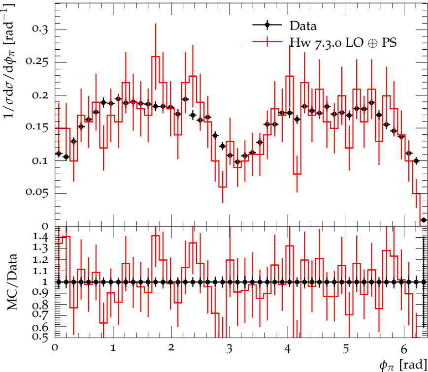
\phi_\pi distribution for \chi_{c0} production with \chi_{c0} \rightarrow \pi^+\pi^-
