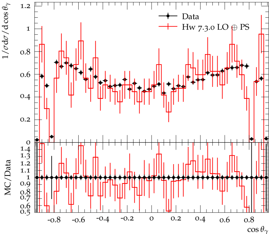
\cos \theta_\gamma distribution for \chi_{c0} production with \chi_{c0} \rightarrow K^+ K^-
